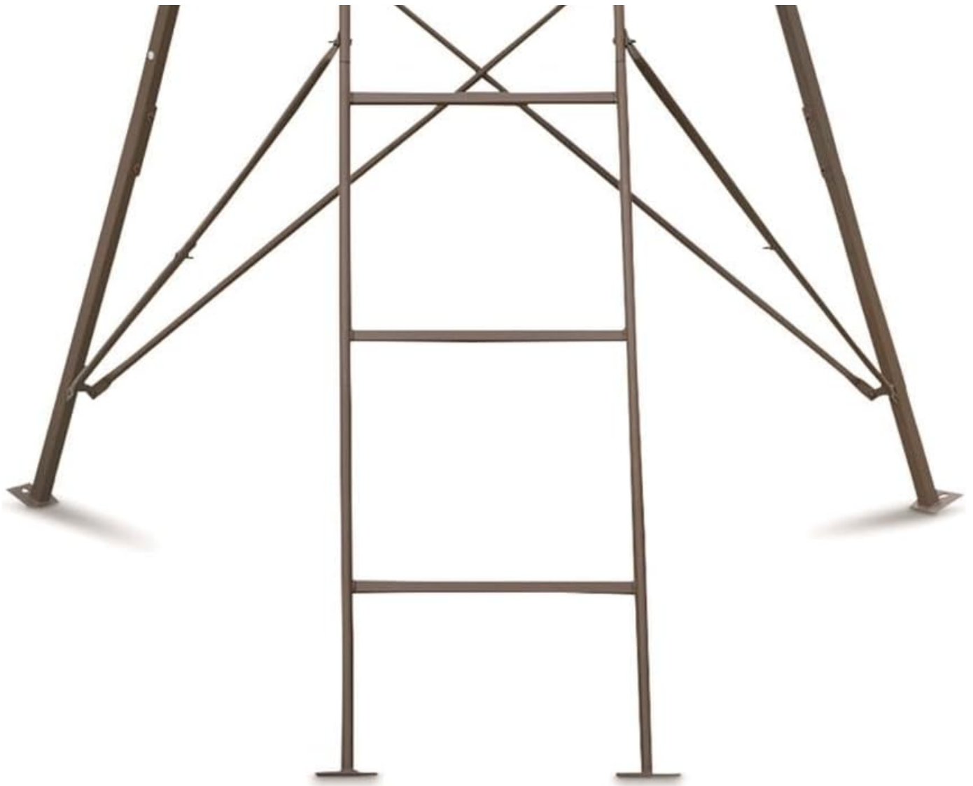
Figure 2: The full steel frame assembled and ready for the blind cover.
