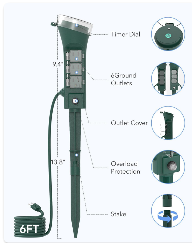
Figure 2: Detailed diagram of the HBN Outdoor Smart Plug components.
