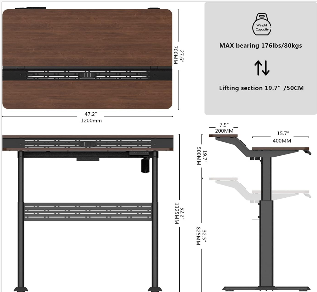
Figure 2: Desk Dimensions and Weight Capacity
