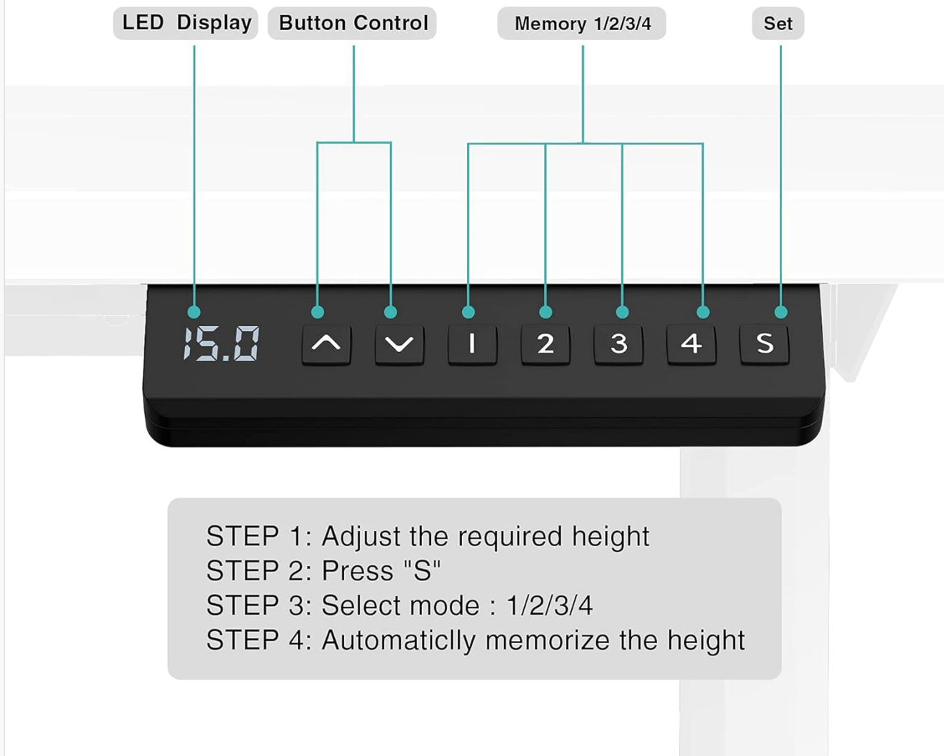
Figure 3: Controller Touch Panel and Memory Setting
