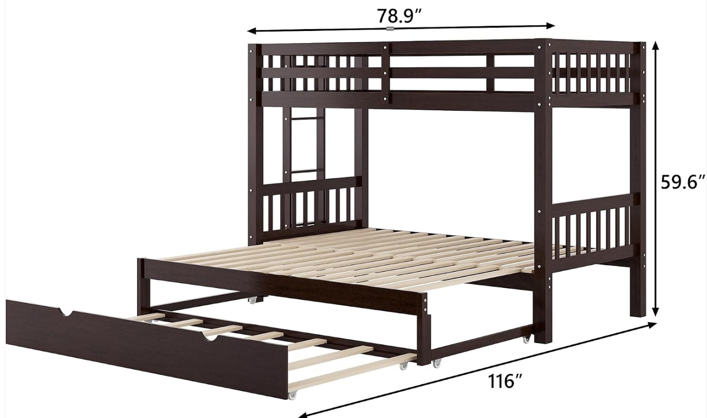
Figure 2: Detailed dimensions of the bunk bed, including height, length, and width.
