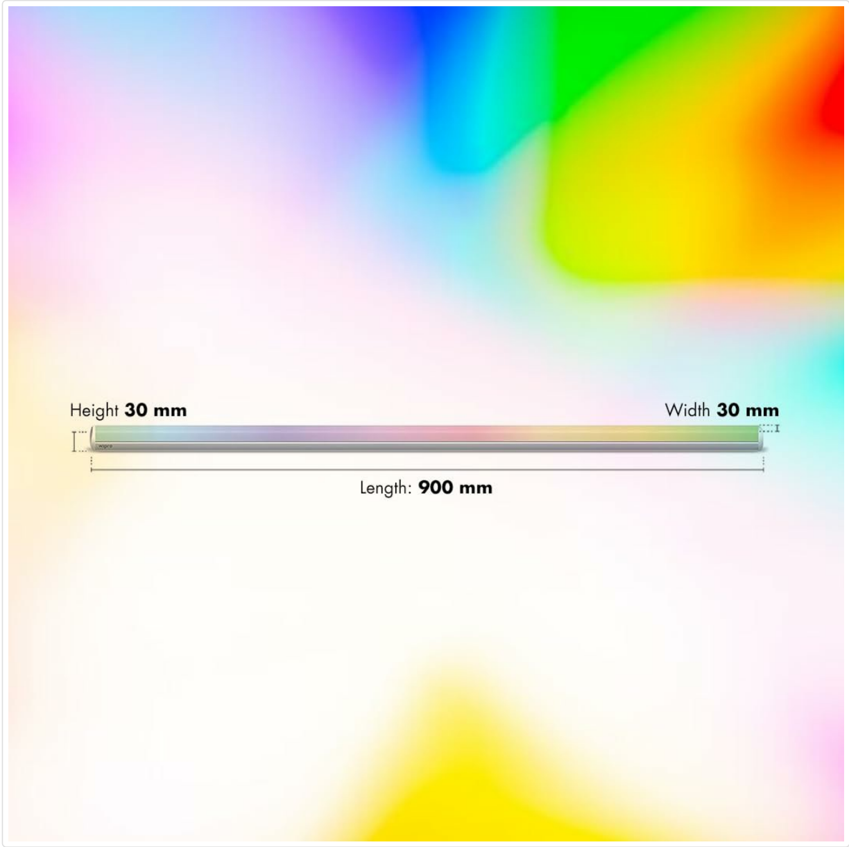
Figure 9.1: Product Dimensions.
