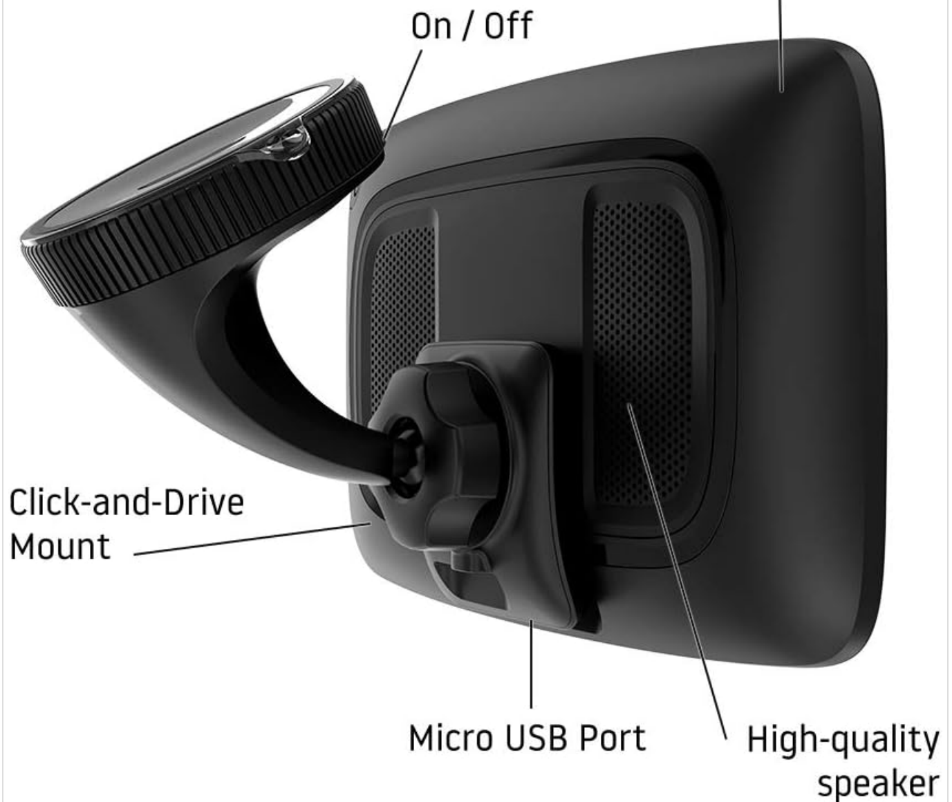
Image: Rear view of the TomTom GO Discover, highlighting the Click-and-Drive Mount, the On/Off button, the Micro USB Port, and the high-quality speaker.
