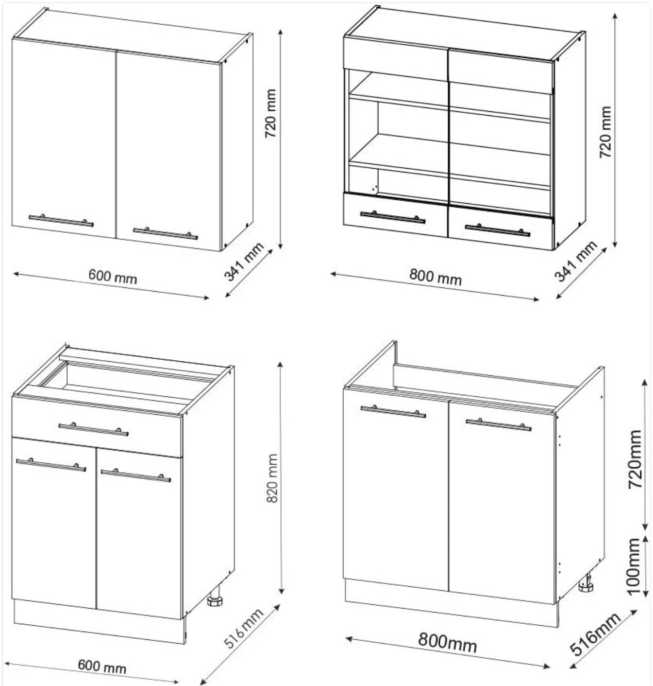
Image: Detailed dimensional drawings illustrating the various cabinet modules and their measurements, crucial for planning and assembly.
