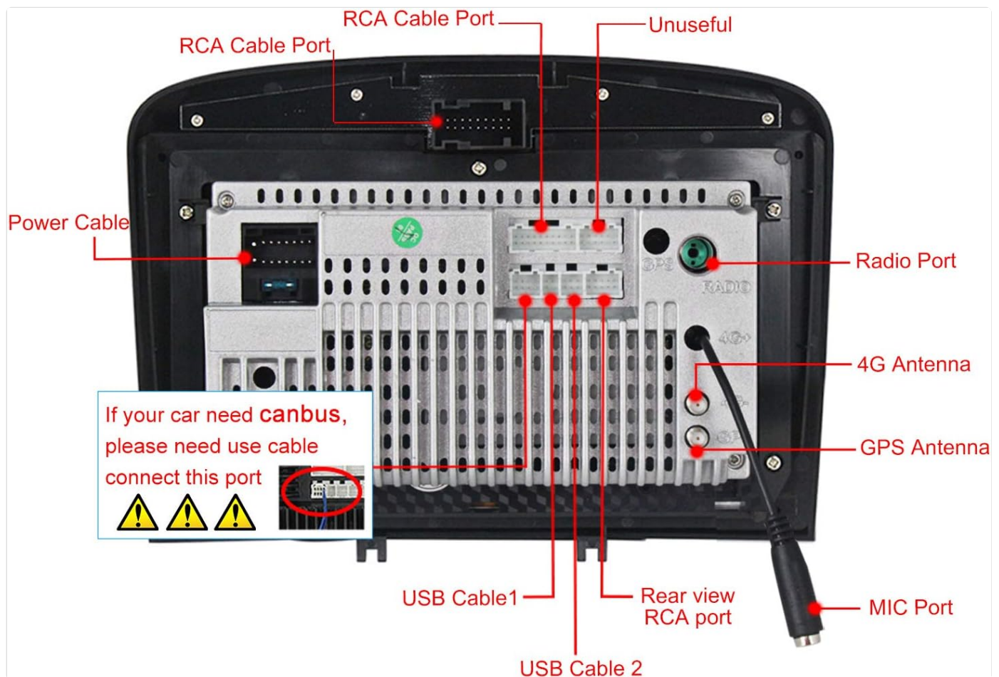
Image: Rear view of the MekedeTech M400 car radio showing labeled ports for power, RCA cables, USB cables, radio antenna, 4G antenna, GPS antenna, and microphone. A note indicates the Canbus connection point.
