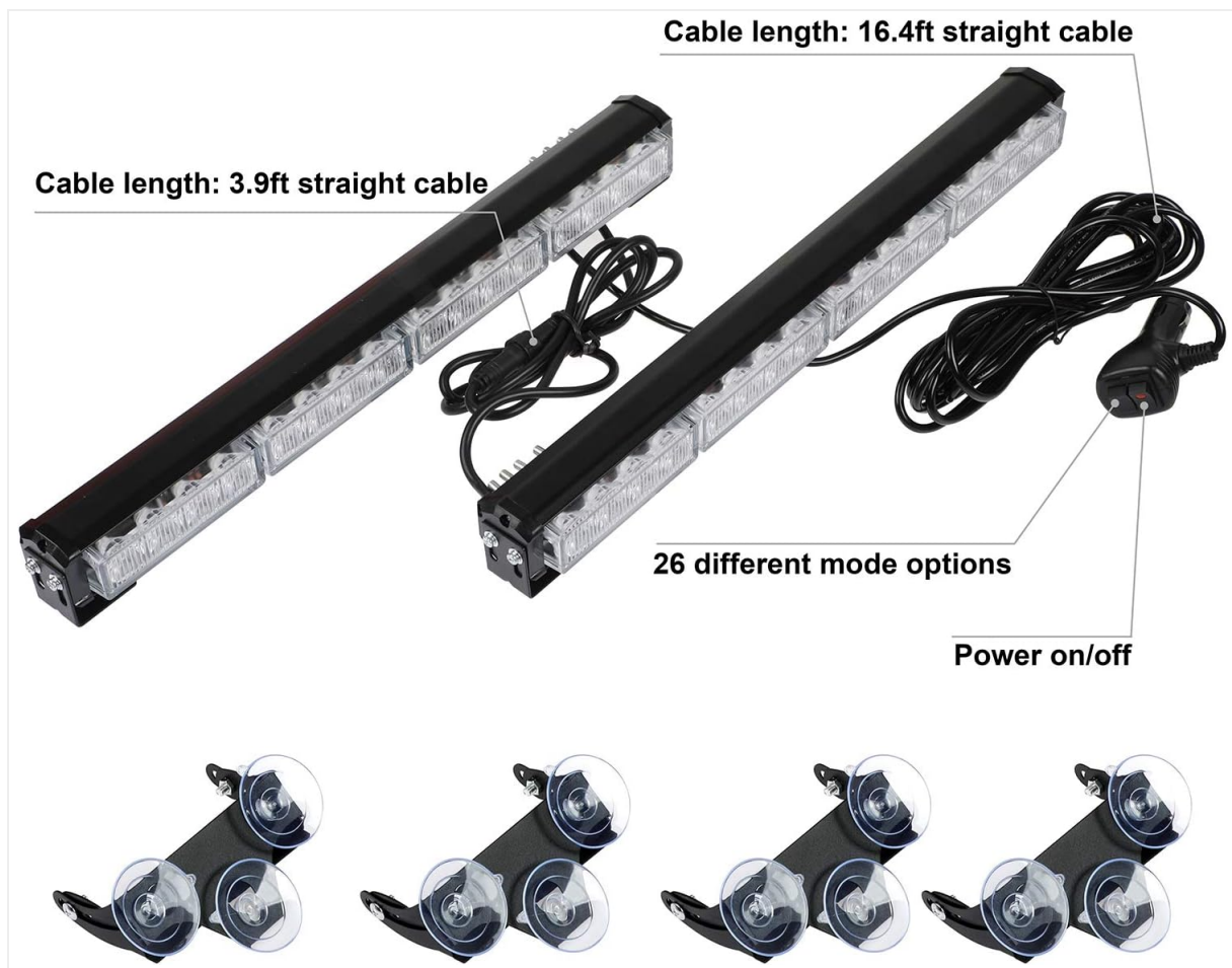
Image 4.3: Detailed view of the light bar wiring, including the 3.9ft light-to-light cable and the 16.4ft power cable leading to the cigarette lighter adapter with dual control buttons.
