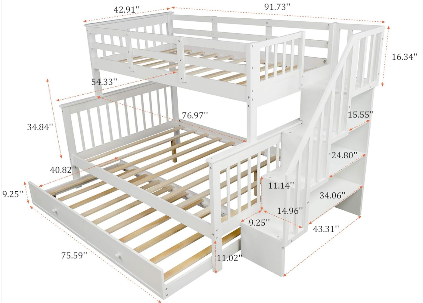
Image: A technical diagram illustrating the precise length, width, and height measurements of the bunk bed, including the trundle and staircase unit.
