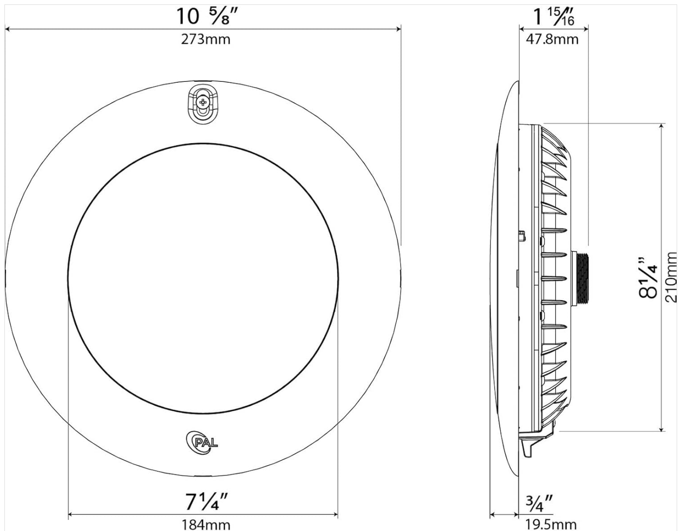
Figure 2: Dimensional drawing of the EvenGlow Pool Light, showing key measurements for installation planning.
