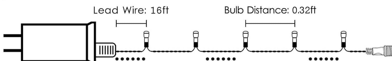
Figure 6: A technical diagram illustrating the total length (180.4ft), lead wire (16ft), and bulb distance (0.32ft) of the 29V 500LED string lights.
