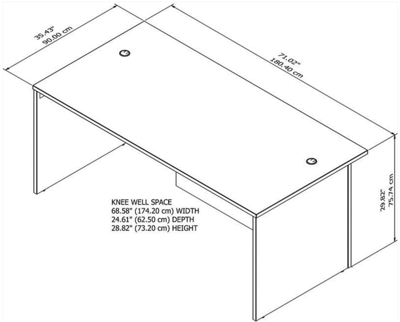
Image 3.1: Desk dimensions and knee well space diagram.
