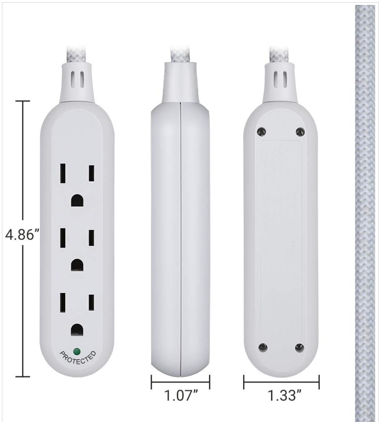
Image: A diagram showing the dimensions of the DEWENWILS 3-Outlet Power Strip, including length, width, and thickness measurements.
