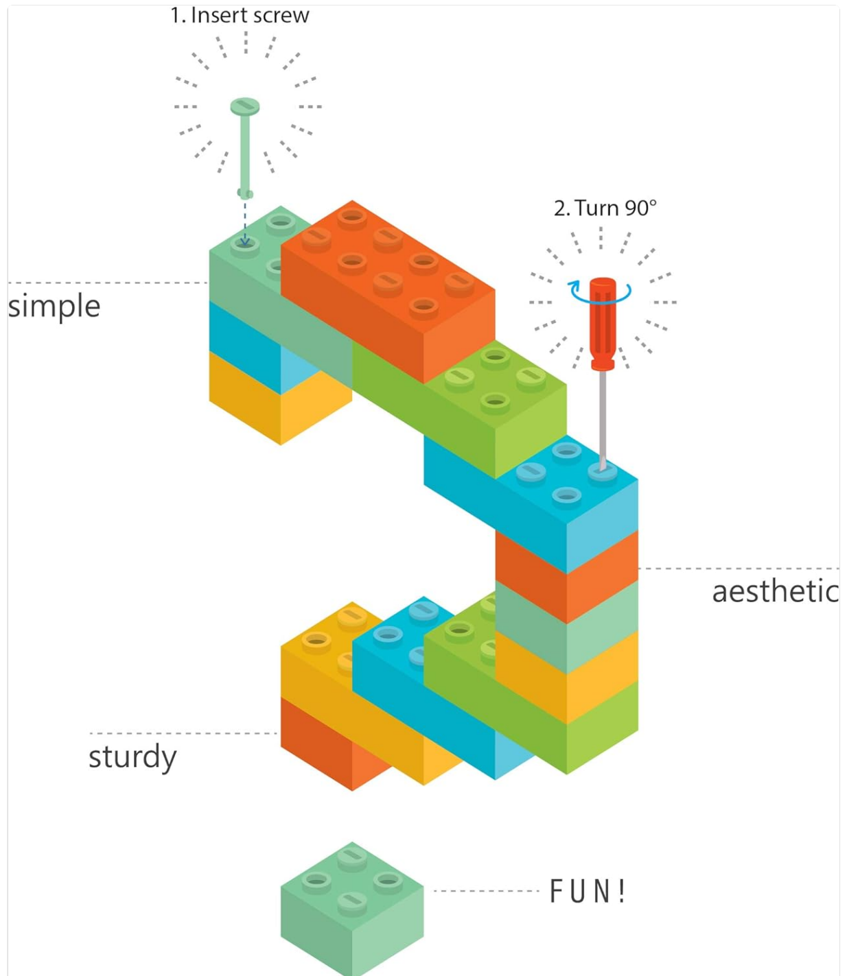
Image: The JEKCA interlocking system. Insert the pin (screw) and turn 90 degrees to secure the bricks, ensuring a sturdy and aesthetic build.
