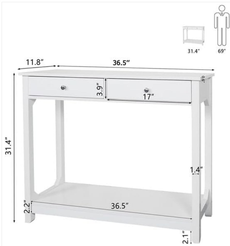
Image: Detailed diagram illustrating the dimensions of the console table, including height, width, and depth.
