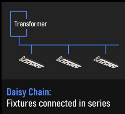
Figure 5: Wiring Configurations
