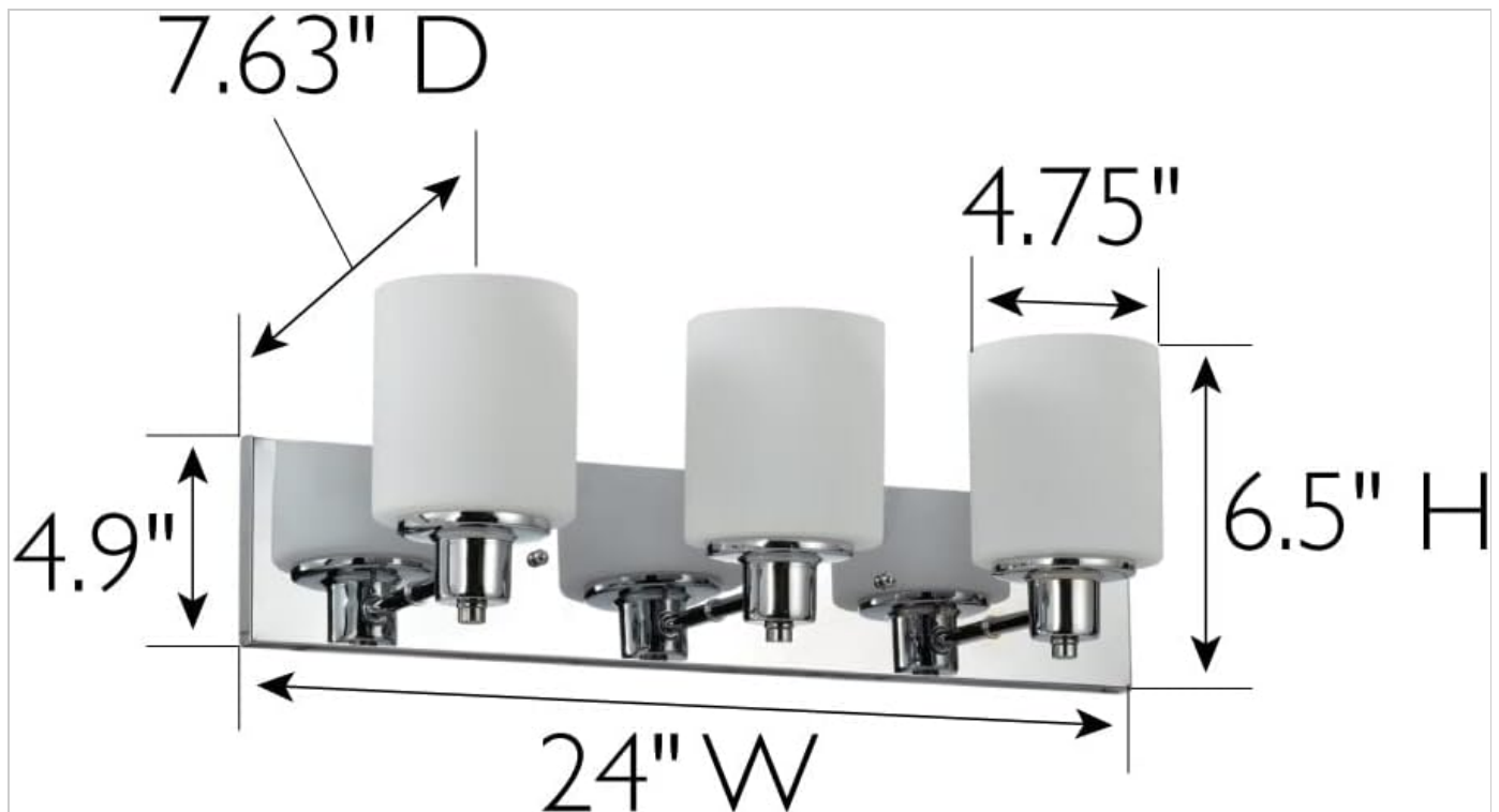
Figure 3: Product Dimensions for planning installation.
