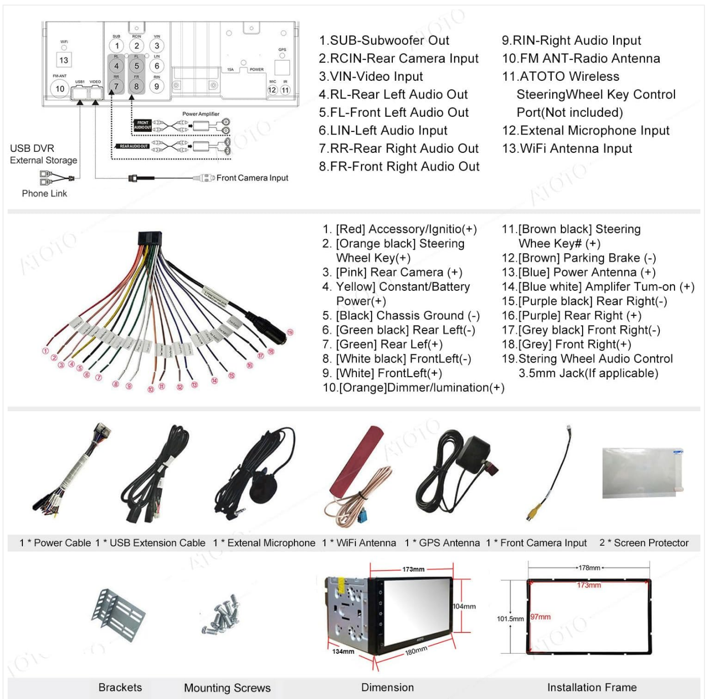
Figure 2.1: All components included in the ATOTO S8 Premium package.
