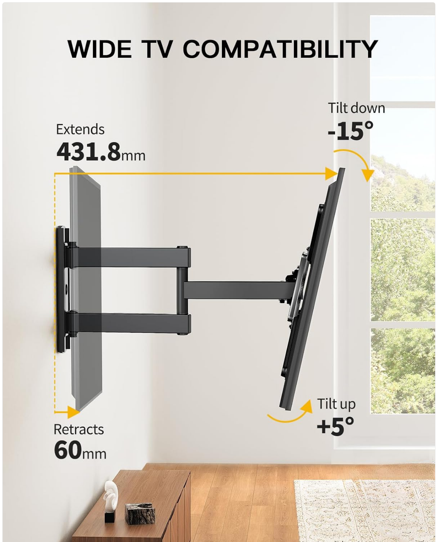
Figure 6: Illustration demonstrating the mount's extension (up to 431.8mm) and retraction (to 60mm) capabilities, along with tilt angles (+5° up, -15° down).
