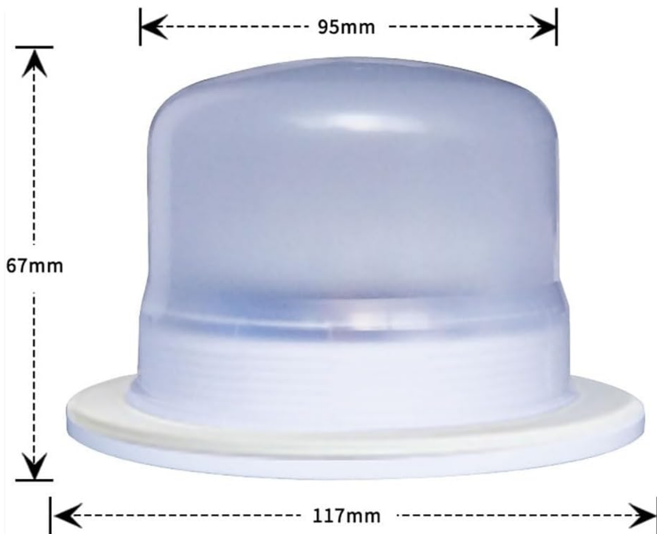
Image 3.2: Dimensional diagram of the LED module, showing a diameter of 117mm and a height of 67mm.
