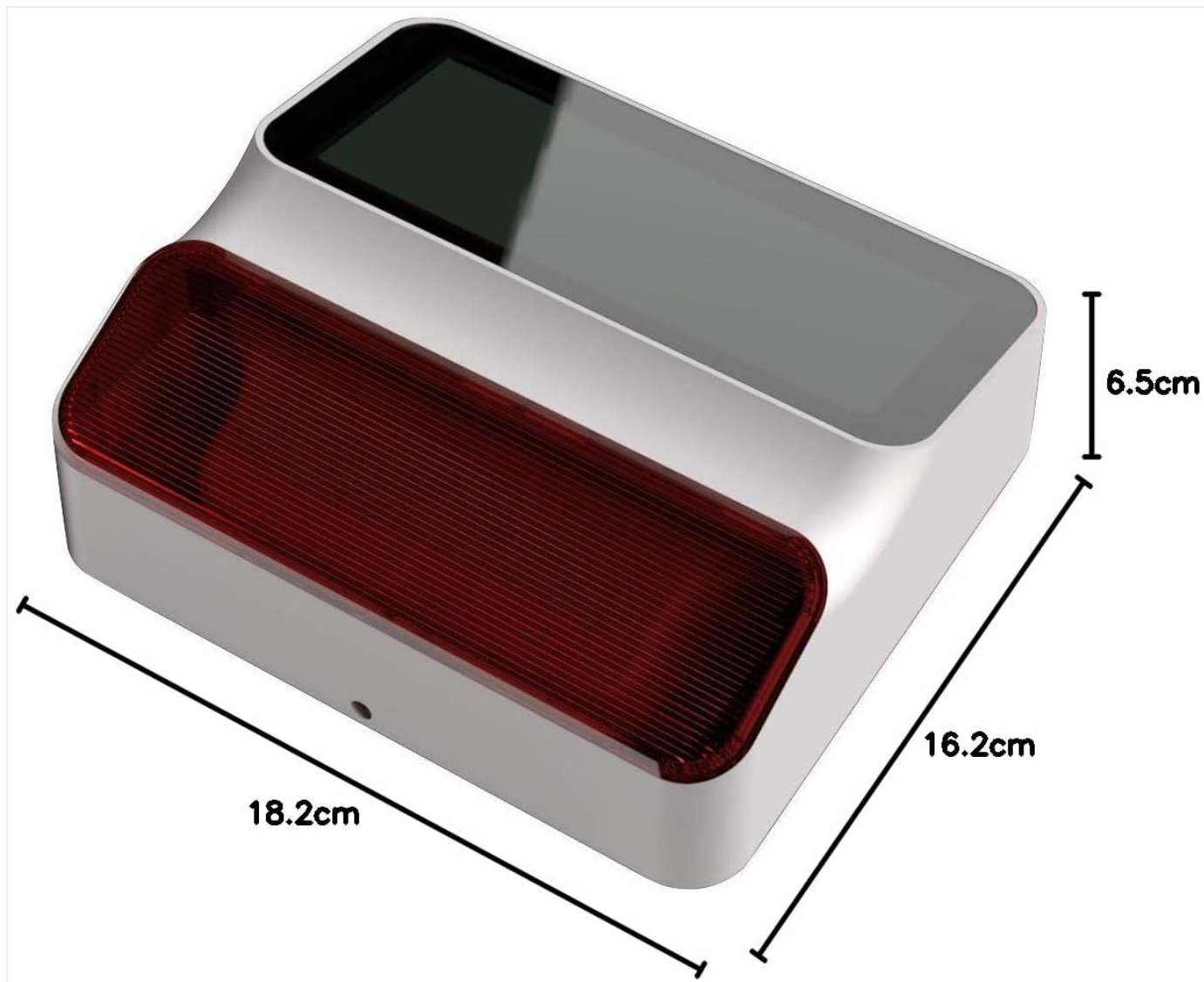
Figure 4.2: Detailed dimensions of the WOS501S siren, indicating its compact size for easy outdoor installation.
