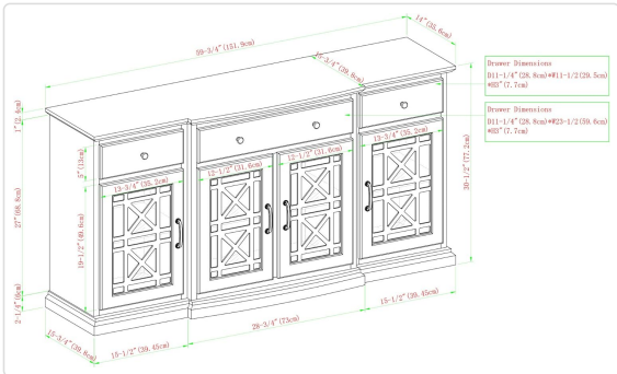
Detailed line drawing of the sideboard, including all key dimensions for planning placement.
