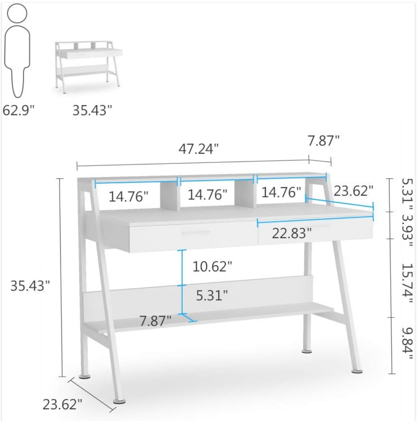
Figure 7.1: Product Dimensions. This diagram provides precise measurements for the desk's width, depth, and height, including the monitor stand and lower shelf.
