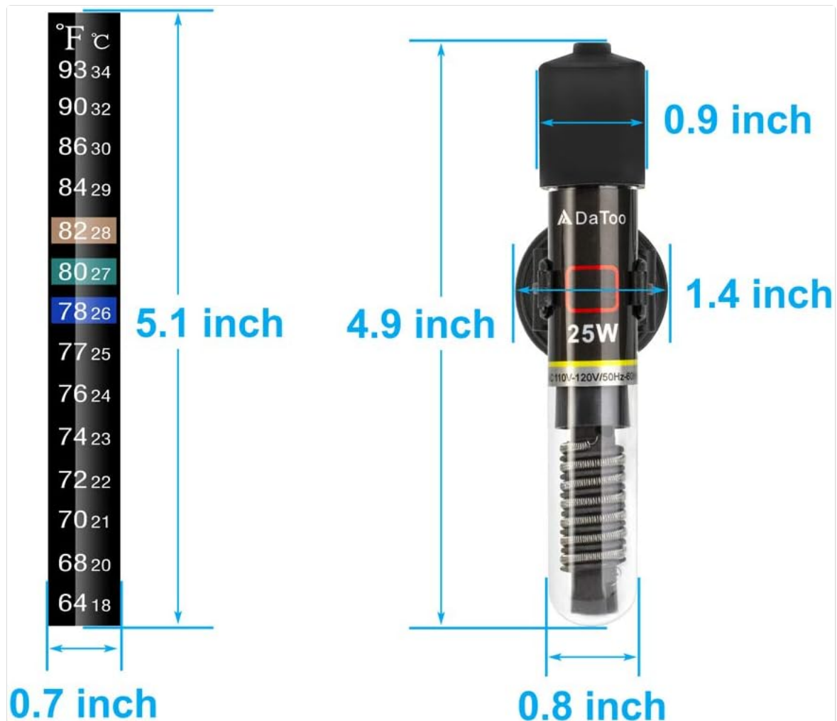
Figure 8.1: Dimensions of the heater and thermometer sticker.
