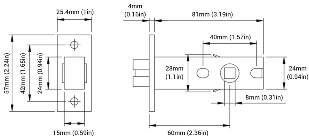
Figure 6.1: Detailed dimensions and adjustable single latch mechanism.
