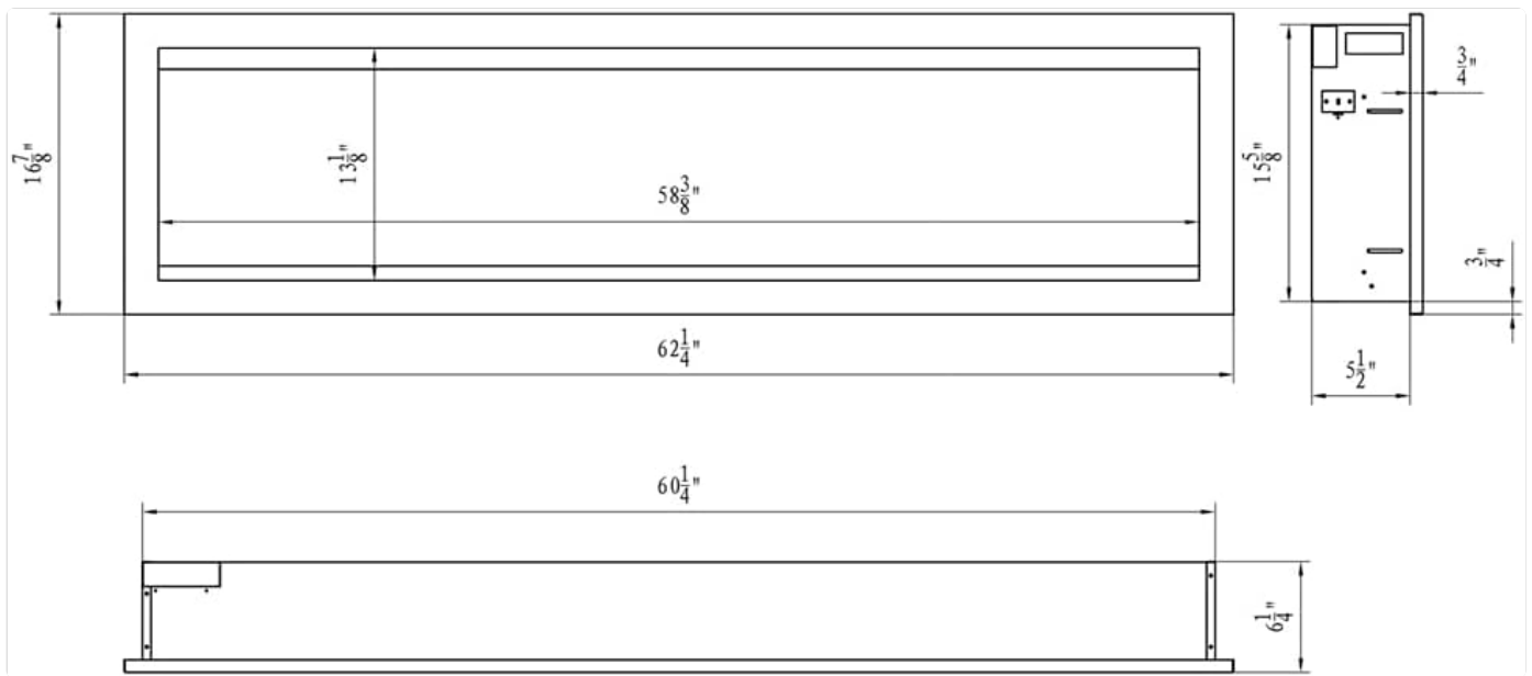
Image: Detailed technical drawing showing the dimensions of the Amantii Symmetry Series Electric Fireplace for installation planning.
