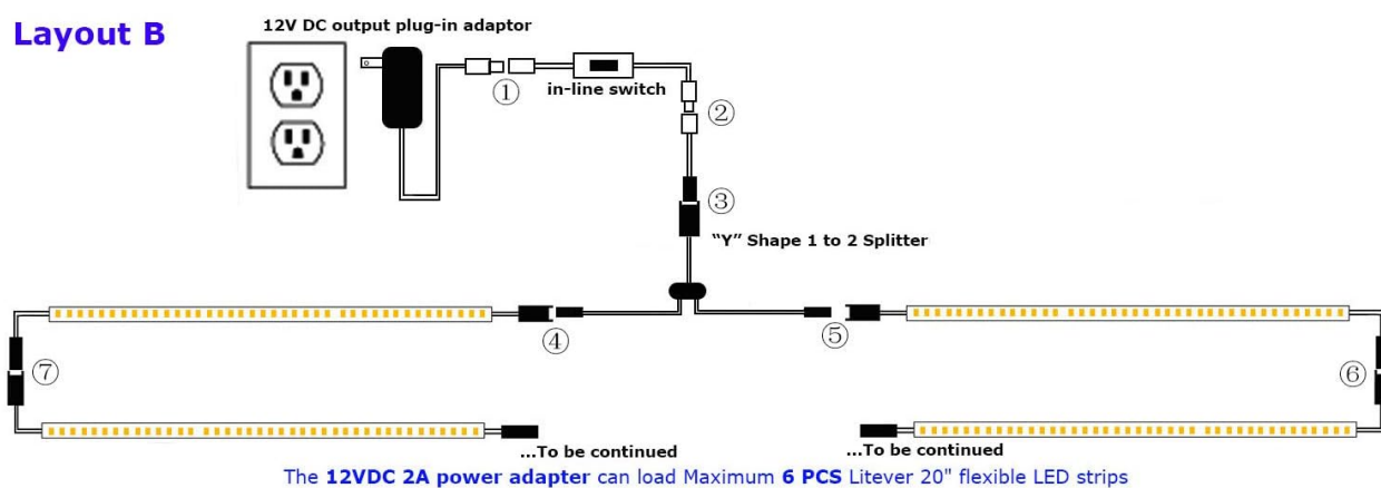
Figure 7: Example wiring layouts for the lighting kit.
