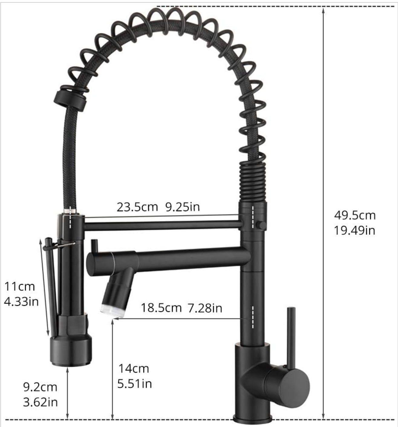
Diagram showing the dimensions of the AIMADI kitchen faucet in centimeters and inches.
