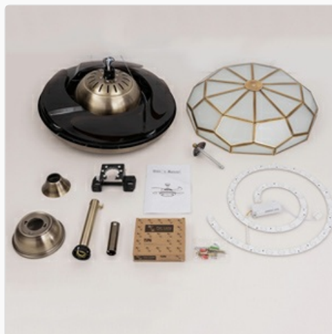
Image 3.1: Overview of the included components for the TFCFL ceiling fan light.
