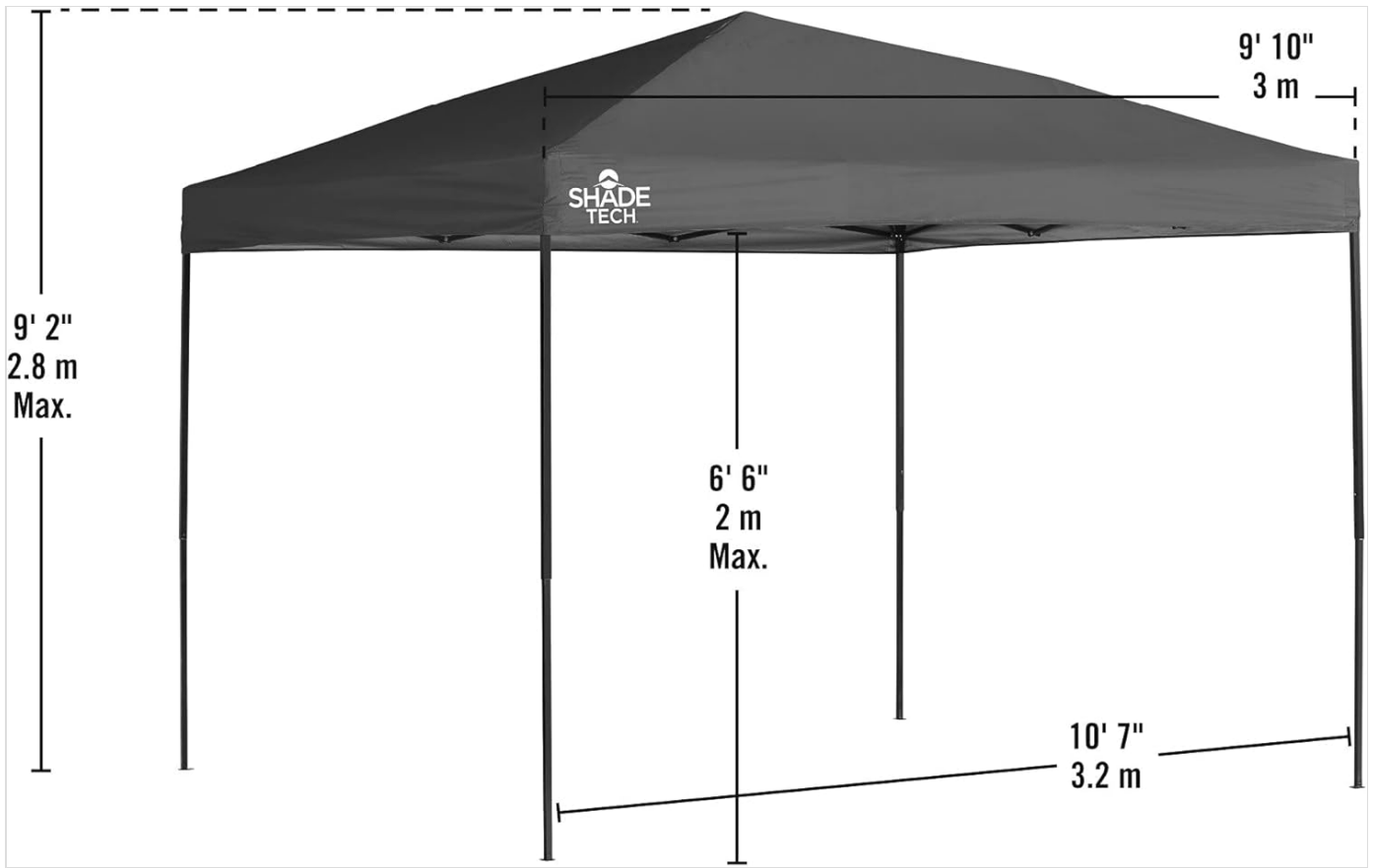
Figure 5: Canopy dimensions.
