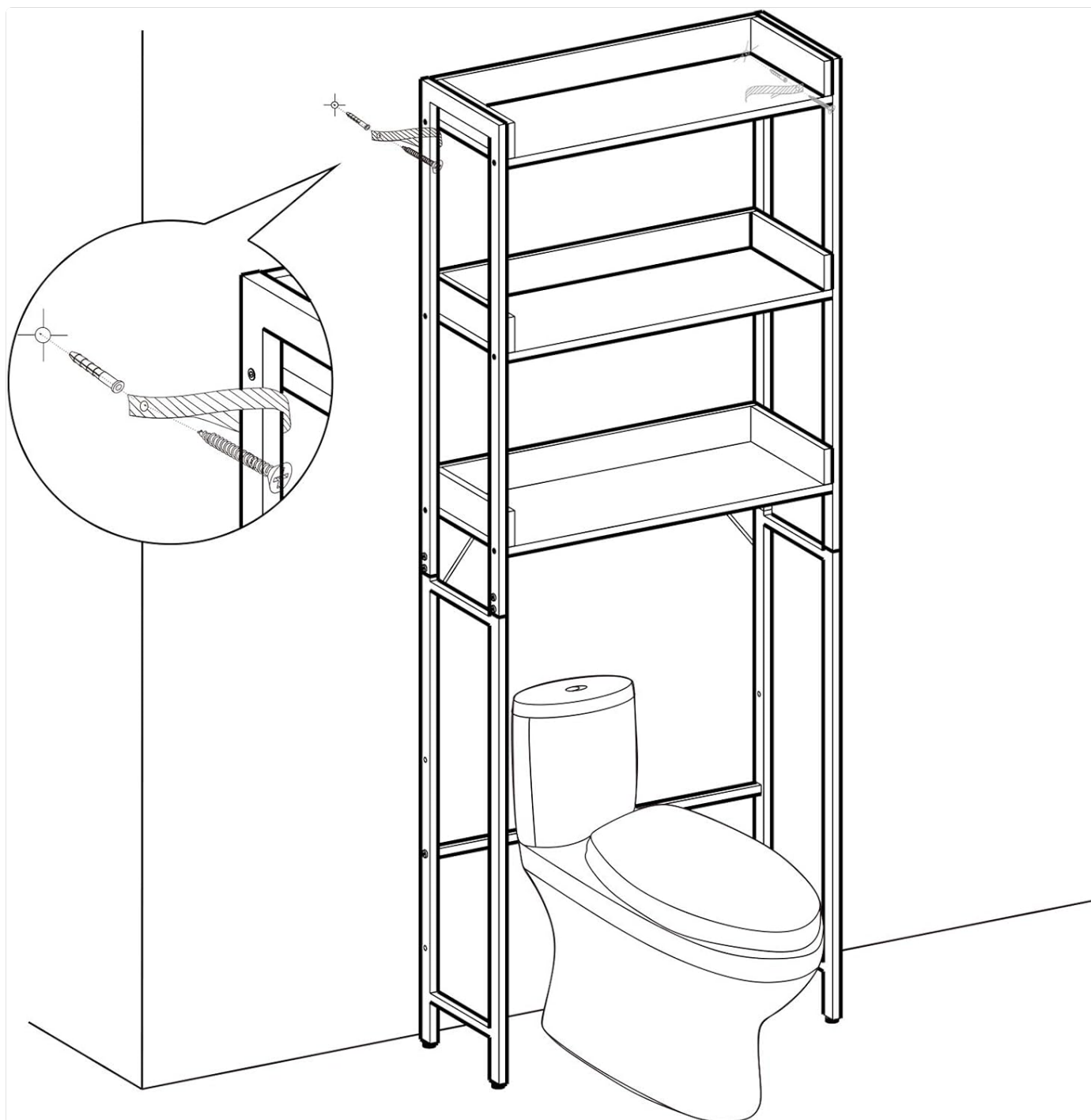
Image: An illustrative diagram showing the assembly process and the installation of the anti-tipping kit to secure the shelf to the wall.
