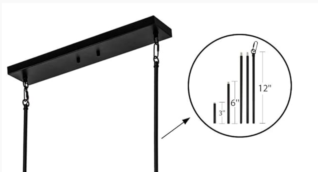
Image: Detail of the adjustable hard stems.
