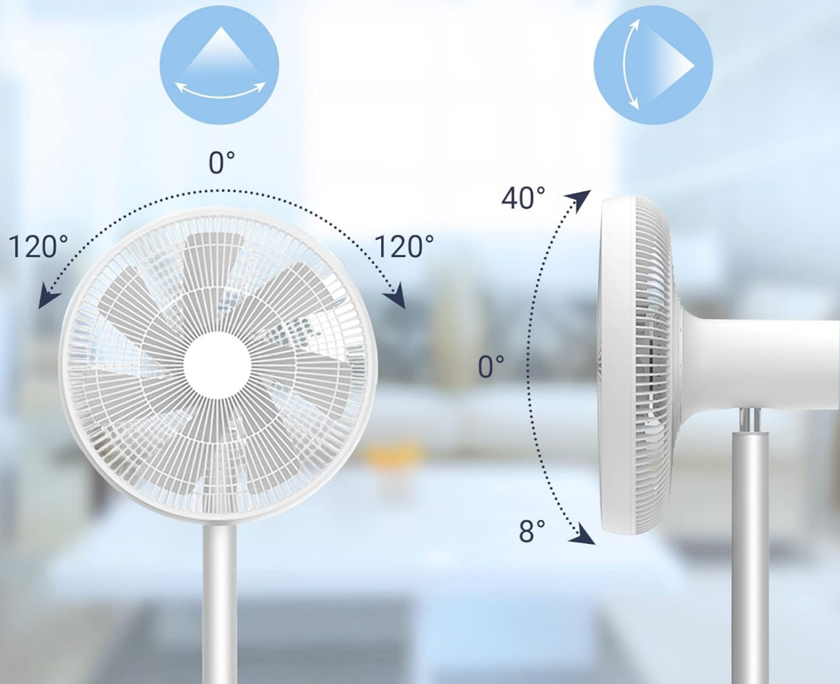
Figure 4: Fan oscillation and tilt capabilities.
