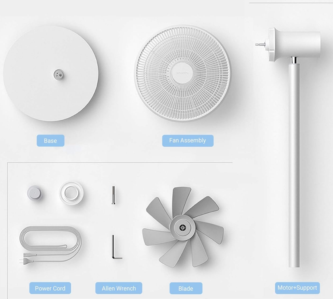
Figure 2: Fan components for easy 5-minute assembly.
