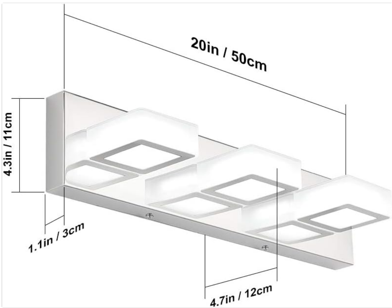
Figure 2: Product dimensions for planning installation space.
