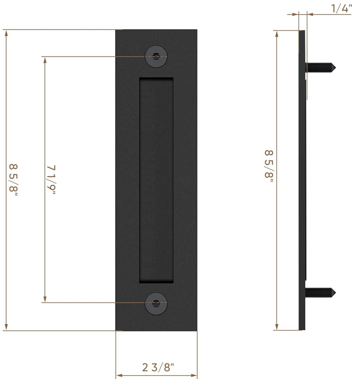
Image 7.1: Detailed product dimensions for the JUBEST handle.
