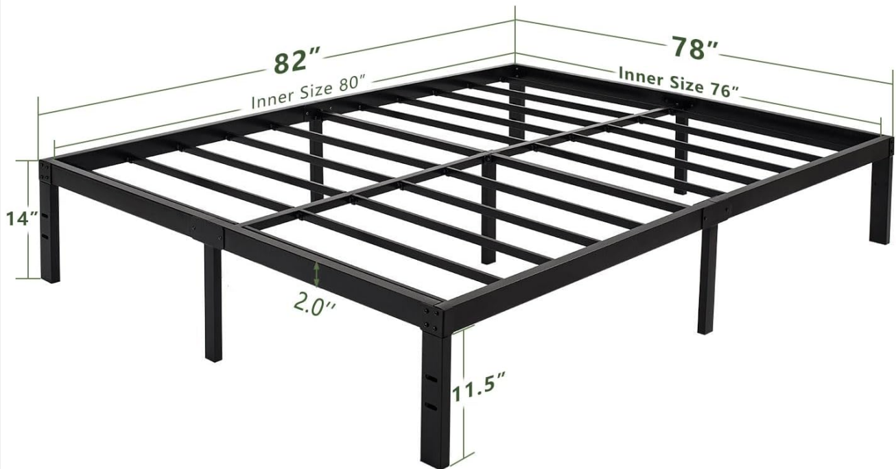
Image: Detailed dimensions of the 45MinST King Platform Bed Frame, including external, internal, and package dimensions.
