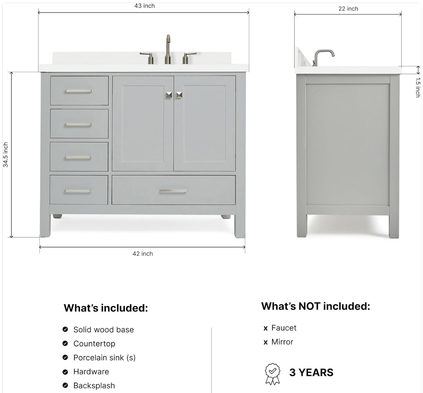
Figure 3: Detailed dimensions of the ARIEL Cambridge 43-inch vanity.
