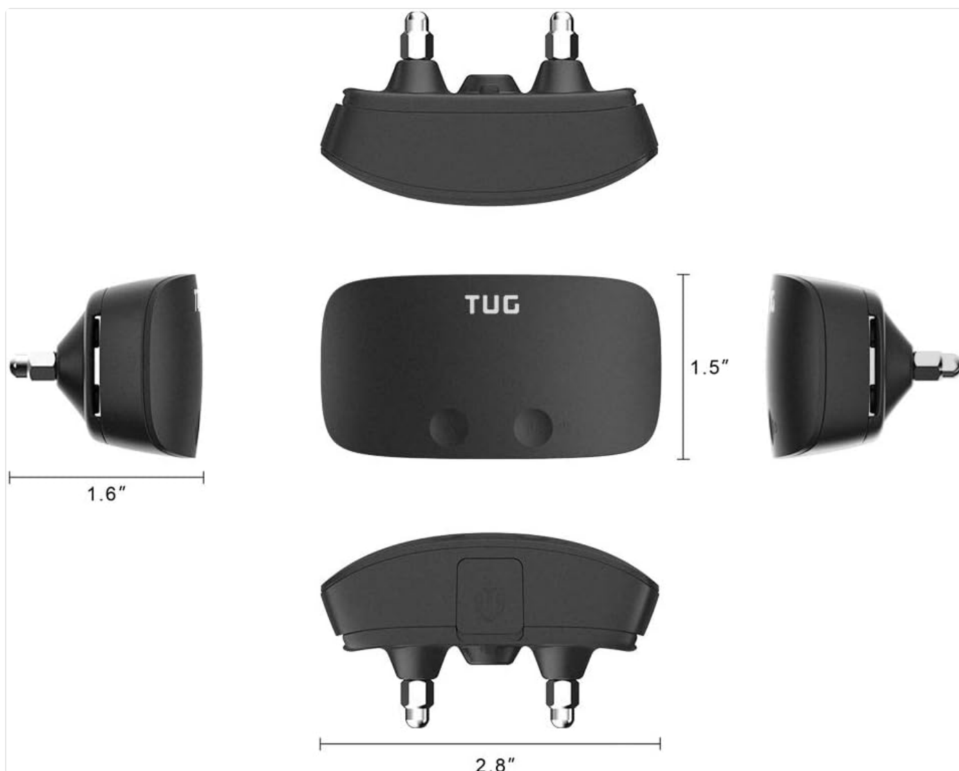
Image: Various views of the TUG Bark Collar with measurements, showing its compact size and dimensions (approximately 2.8" length, 1.6" width, 1.5" height).
