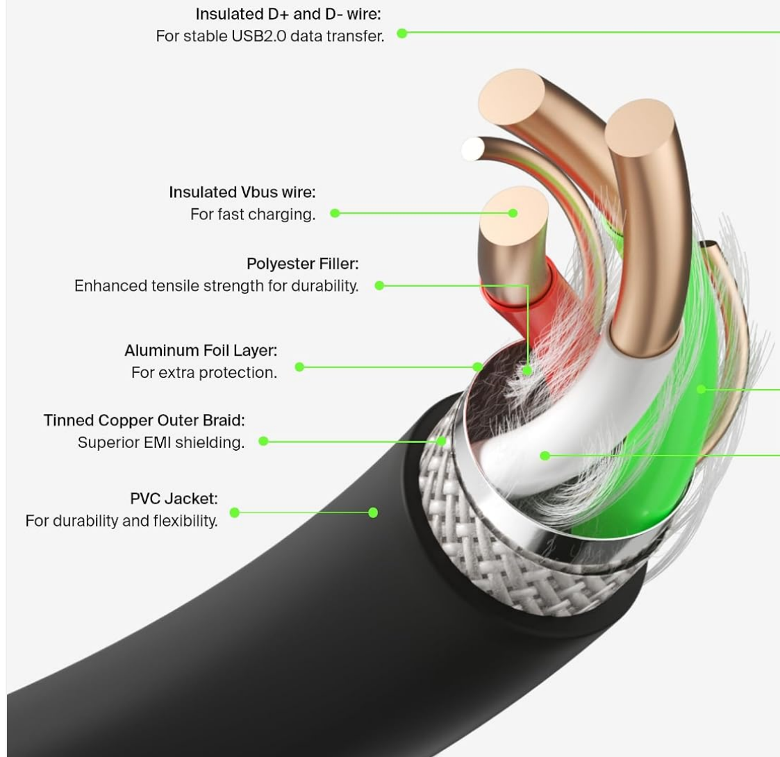
Figure 5: Internal construction of the cable, engineered for safety and performance.
