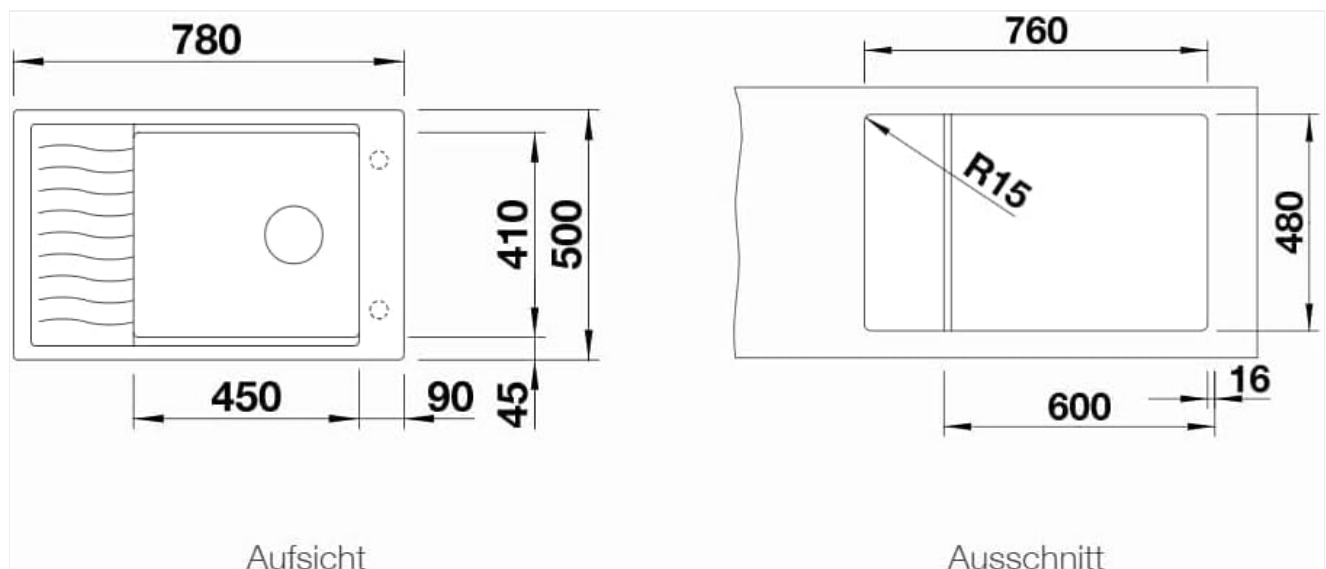
Figure 2: Top view dimension diagram for the BLANCO Elon XL 6 S sink, showing overall length (780mm), width (500mm), and bowl
