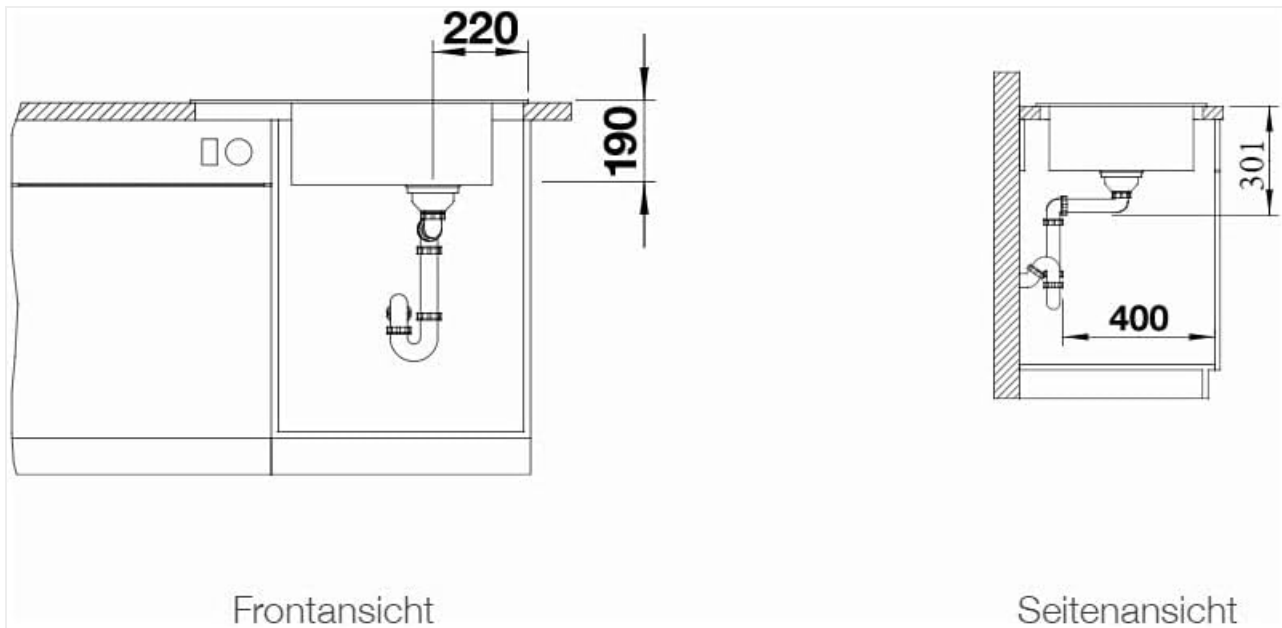
Figure 3: Front and side view dimension diagrams for the BLANCO Elon XL 6 S sink, indicating depth (190mm) and required under-counter space.
