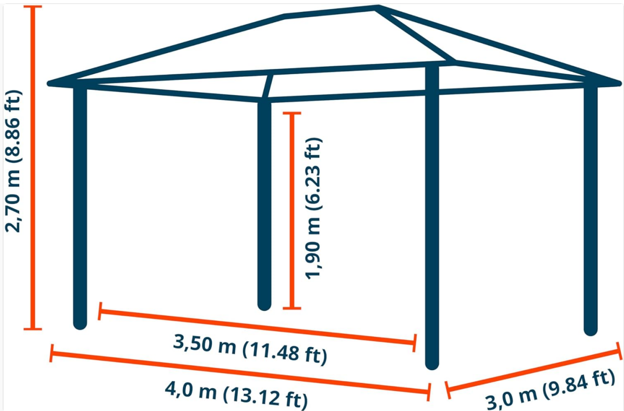
Figure 2.2: Dimensional diagram of the 10x13 ft gazebo. Dimensions are approximately 4.0 m (13.12 ft) length, 3.0 m (9.84 ft) width, 2.70 m (8.86 ft) total height, and 1.90 m (6.23 ft) entry height.
