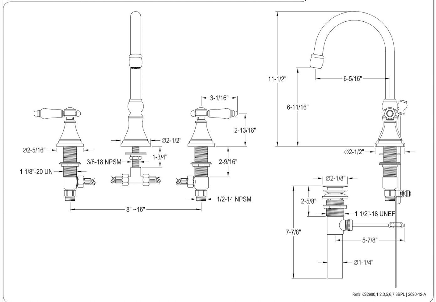
Image: Technical diagram illustrating the dimensions and installation requirements for the Kingston Brass Widespread Lavatory Faucet series, including the KS2982BPL model. This diagram shows the spout height, reach, handle spacing, and connection types.
