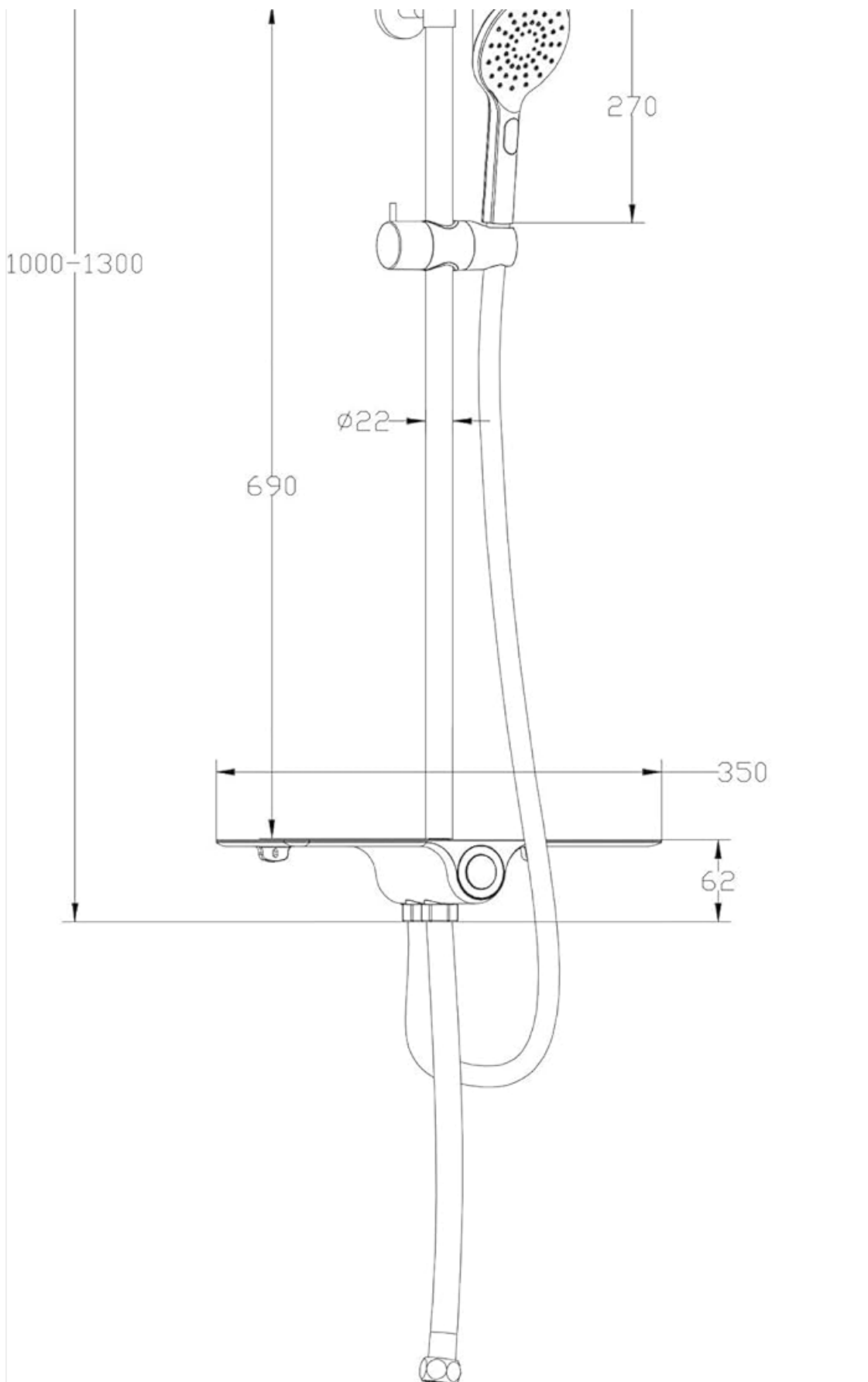
Image: Technical drawing showing the dimensions of the SCHÜTTE AQUASTAR 60520 shower system, including adjustable height and shower head sizes.
