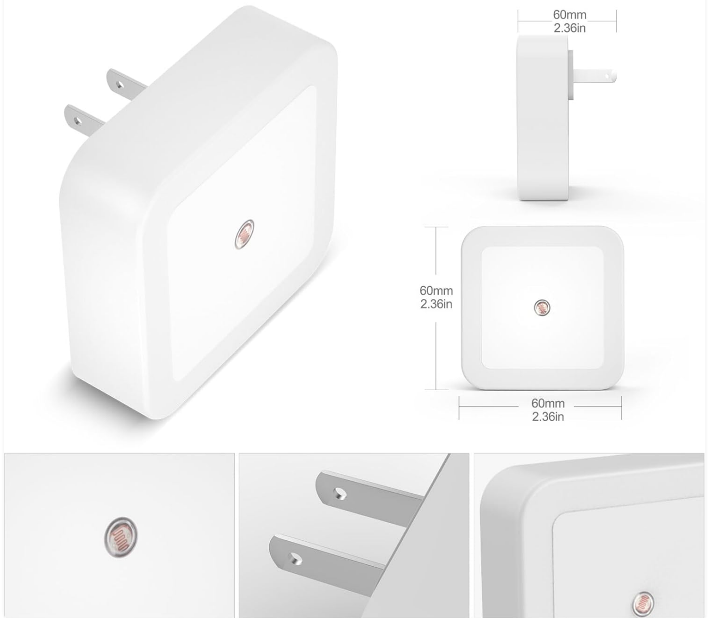
Figure 2: Product Dimensions
