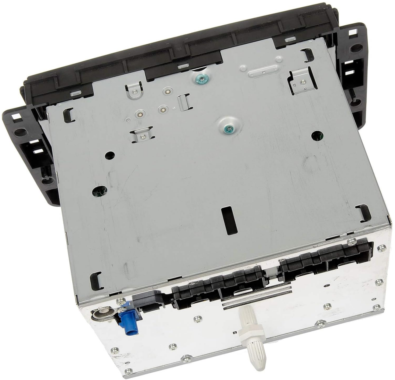
Figure 3: Top and rear view of the module, showing the metal casing and various mounting points.
