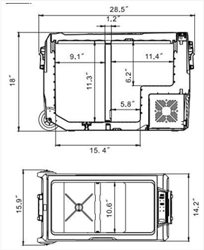
Image: Technical drawing illustrating the external and internal dimensions of the Alpicool T50 portable car refrigerator.
