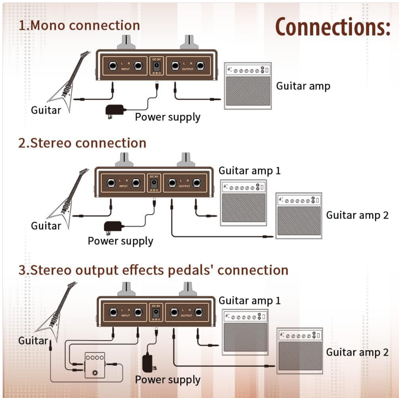
Figure 1: Connection diagrams for mono, stereo, and stereo output effects pedal setups.
