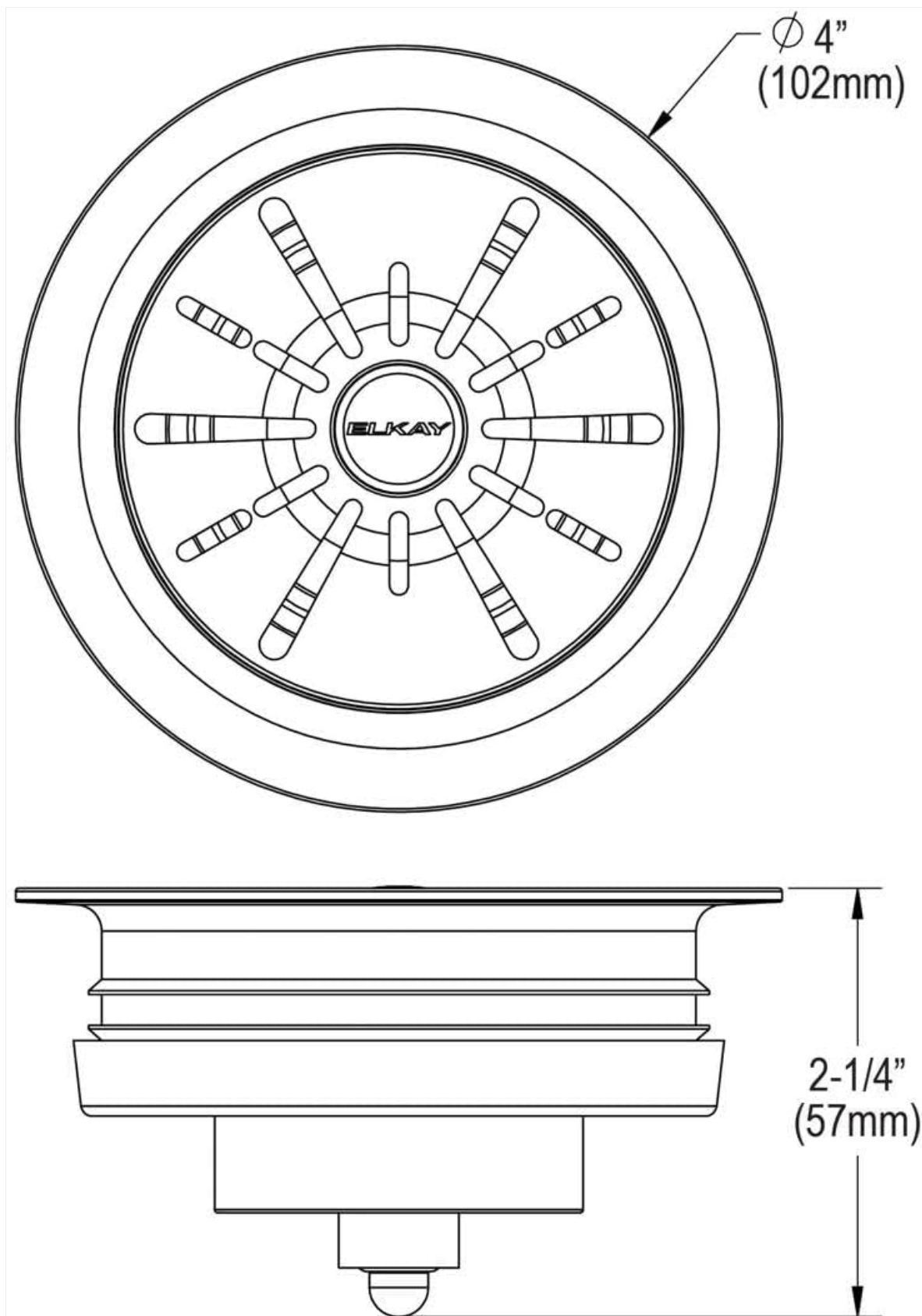
Image: Technical drawing showing the dimensions of the Elkay Perfect Drain Disposer Flange, including a 4-inch (102mm) diameter and 2-1/4 inch (57mm) height.
