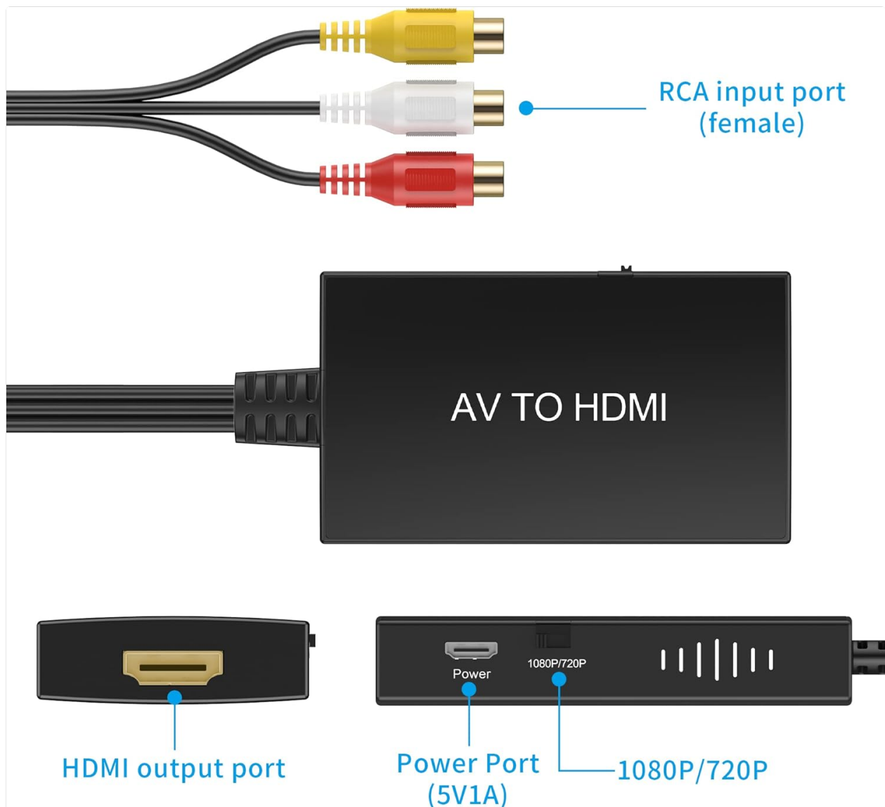
Figure 4: RCA input ports (Yellow, White, Red) on the converter.
